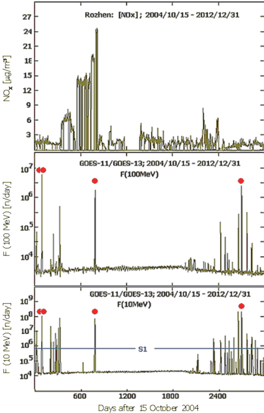
Figure 3: Daily average values of NO_x concentration and daily total flux of the high energy protons - F \geq 100MeV (middle panel) and low energy protons - F \geq 10MeV (bottom panel).
