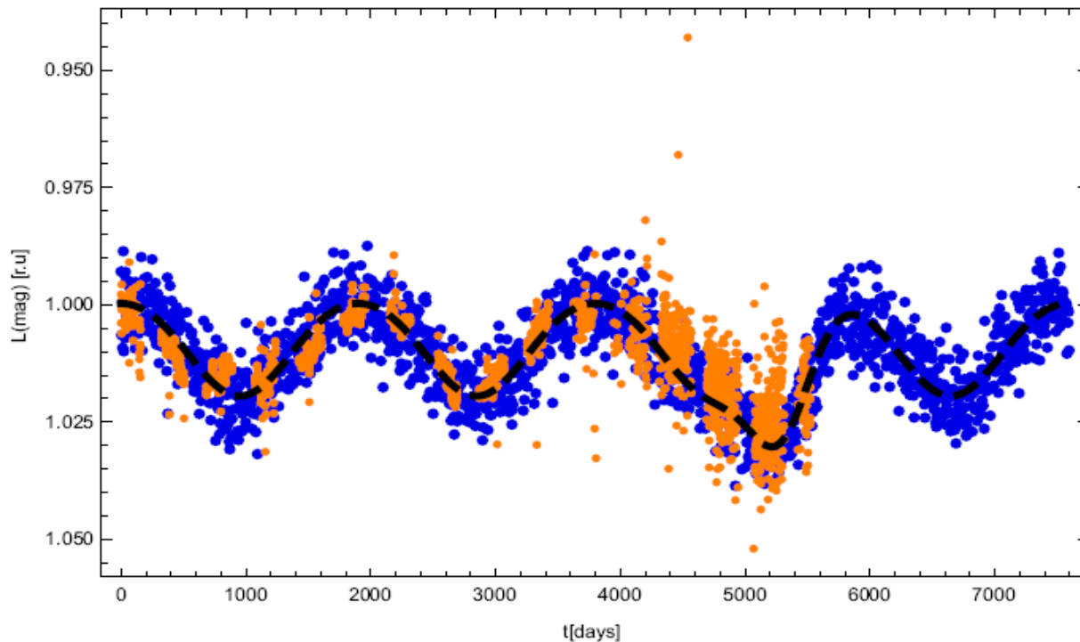
AN INTERPRETATION OF VARIABILITY OF PG1302-102
